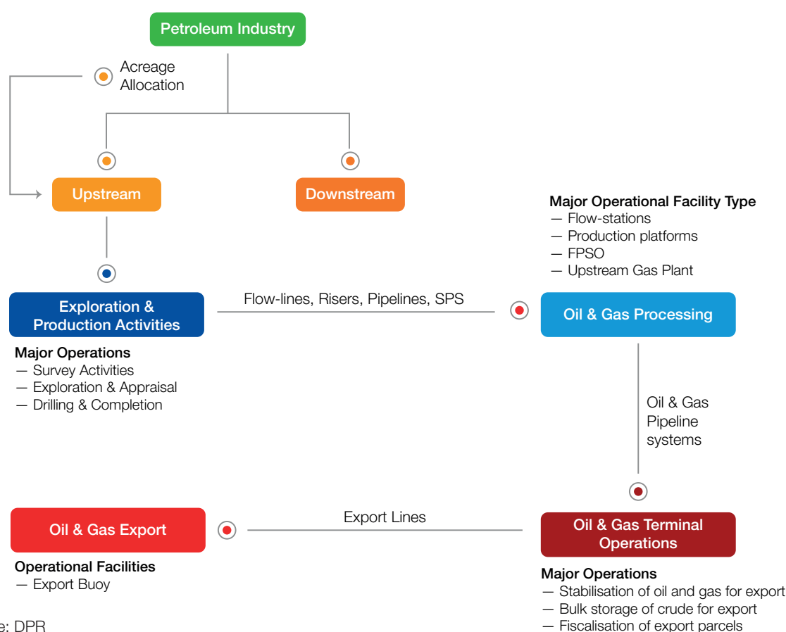
Figure 5 - Flow of Production to Exports
